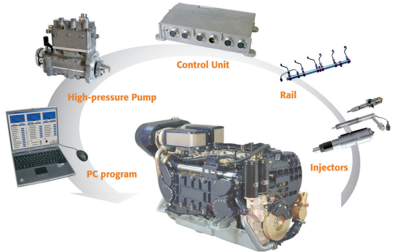
ODYSSEUS – the complete Common Rail Fuel Injection System
