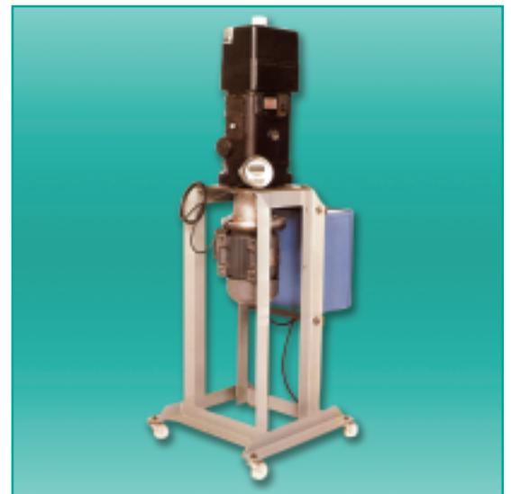
GOVERNOR TEST STANDS Series AK7 Mobile Variable Speed Governor Test Stand
